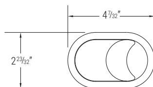
RACETRACK GROMMET (G11)
